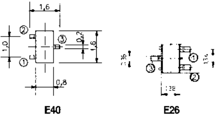
E25/TO-236/SOT-23
